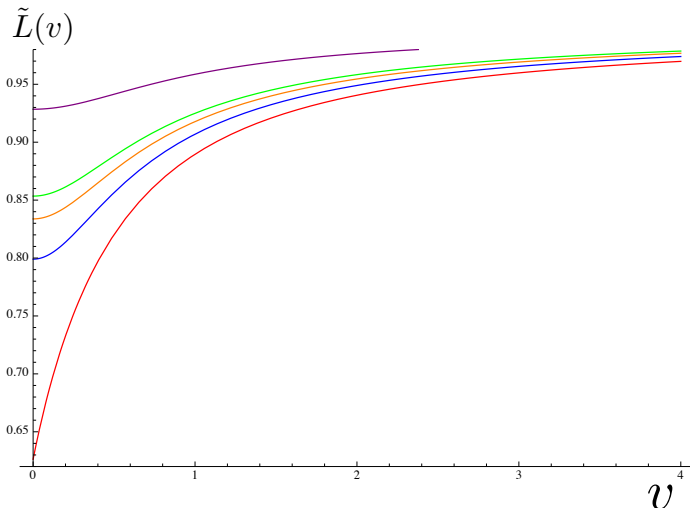
Figure 11: The shape of the D5-brane in the AdS black hole background. Each curve is with r_{\text{H}}/r_{\text{cr}} = 0.9, 0.99, 1, 1.01, 1 respectively from top to bottom. The D5-brane of the red curve has a cusp at \rho = 0 , which we call a critical embedding, for r_{\text{H}} = r_{\text{cr}} (\simeq 0.443) . The other curves are Minkowski embeddings.
