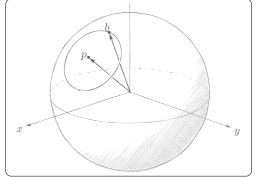
Figure 1: The space L_1 S^2 \subset LS^2 (22) of small loops in the sphere is homotopy equivalent (by Prop. 4.13) to its further subspace of loops that trace out round circles on S^2 , once at constant rate.
