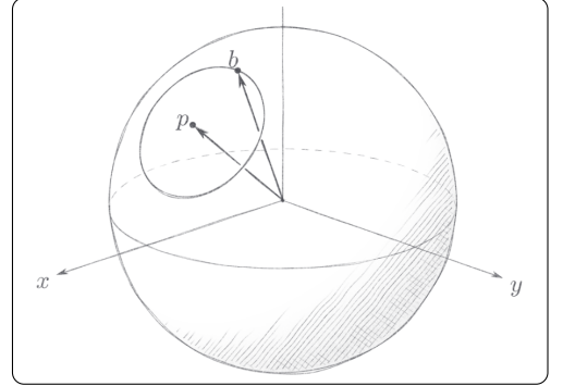
Figure 1: The space L_1 S^2 \subset LS^2 (22) of small loops in the sphere is homotopy equivalent (by Prop. 4.13) to its further subspace of loops that trace out round circles on S^2 , once at constant rate.
