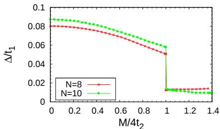
Energy gap
