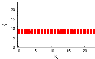
Laughlin on torus \nu = 1/3
