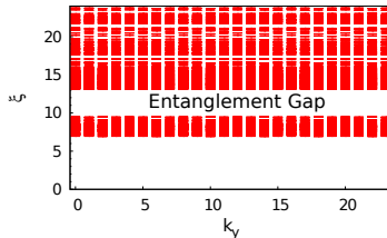
Coulomb on torus \nu = 1/3
