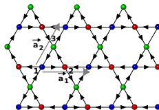
Kagome lattice, E. Tang et al. PRL (2011)
