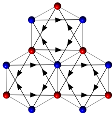
Haldane model, Neupert et al. PRL (2011)
