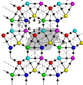
Ruby lattice, PRB (2011)
