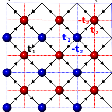
Checkerboard lattice, K. Sun et al. PRL (2011).
