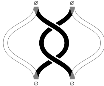
Figure C. In the traditional picture of anyon braiding processes implementing topological quantum computations (e.g. [Kau02, Fig. 17][FKLW03, Fig. 2][NSSFD08, p. 10][Ro16, Fig. 2][DMNW17, Fig. 2][RW18, Fig. 3][Ro22, Fig. 1]), the computation is:
