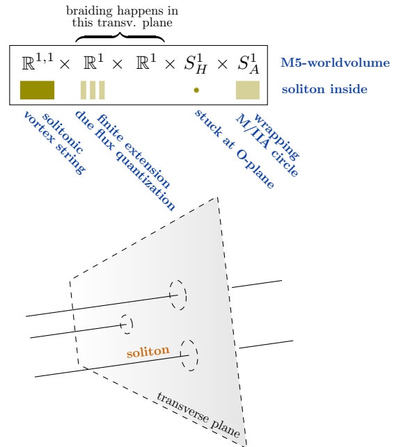
Figure 1. The brane-diagram of the solitons on M5-branes which carry anyonic quantum observables under Hypothesis H. Here, from right to left:
