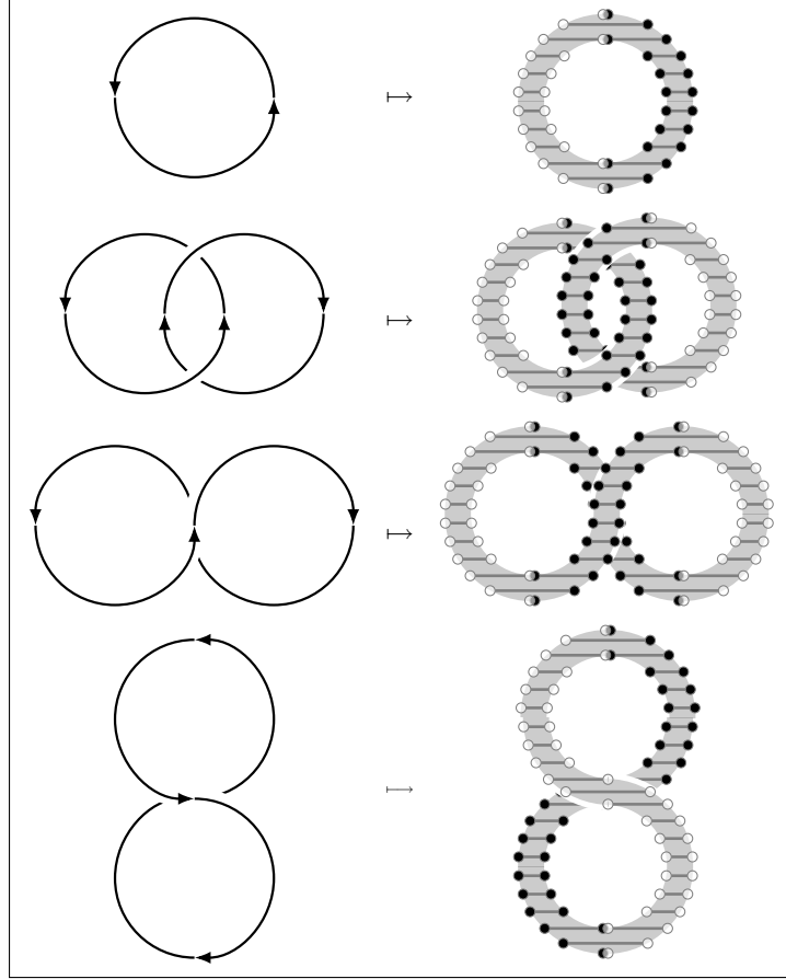
Figure F – Charged string loops as framed oriented links. Notice how it is the stringy nature of the loops of configurations on the right (via Def. 3.3) that reflects the “black-board framing” of the link diagrams on the left. This framing would be absent for configurations of charged points as on the left of Figure 2.
