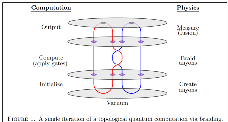
FIGURE 1. A single iteration of a topological quantum computation via braiding. Figure from Rowell ([103], following [102, Fig. 2]).
