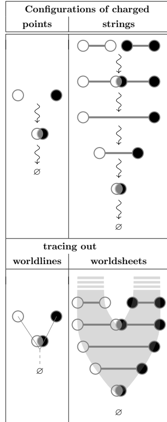
Figure 8: The continuous relations in configuration spaces of charged points and strings exhibit the pair annihilation/creation of oppositely charged (end-)points.
