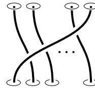
Figure 14: Topological rotation gates , obtained by cyclic braiding of defect anyons, combined with the global phase rotations given by braiding of solitonic anyons, would provide intrinsically exact and topologically protected gates of the kind that make up the quantum Fourier transform (in qdit-bases), and with it many other quantum algorithms.
