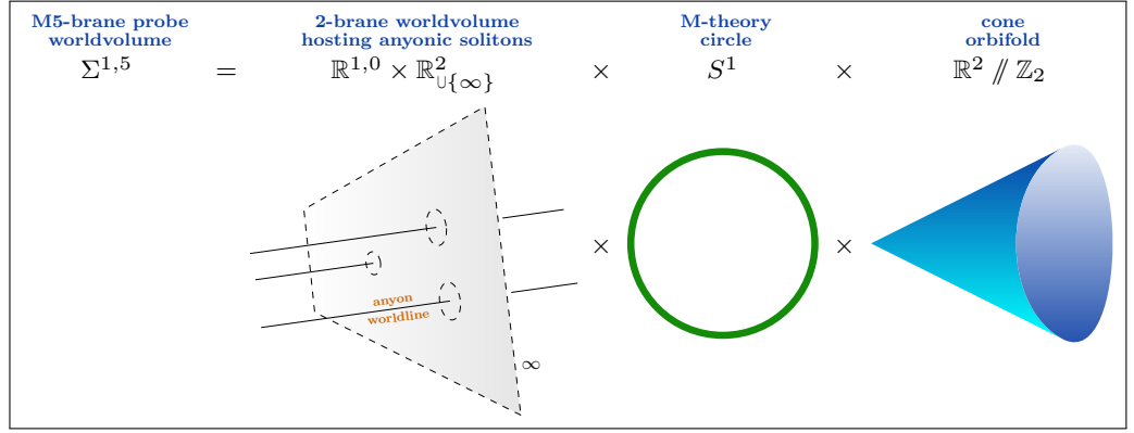
Figure 4: Brane diagram for geometric engineering of anyons on single M5-branes wrapping an orbifold singularity [137]. It is a subtle mechanism of flux-quantization [132] of the self-dual tensor-field on the M5 [54] that stabilizes [134] its anyonic soliton configurations.
