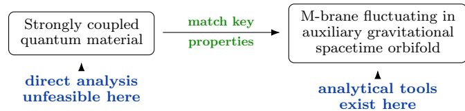
Figure 3: Geometric engineering of quantum systems on M-branes provides tools for analyzing otherwise elusive strongly coupled/correlated quantum phenomena.
