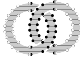
Figure 6: Framed links as stringy worldsheets are revealed by careful analysis as being the loops in the moduli space of solitonic cohomotopy charges of the plane.
