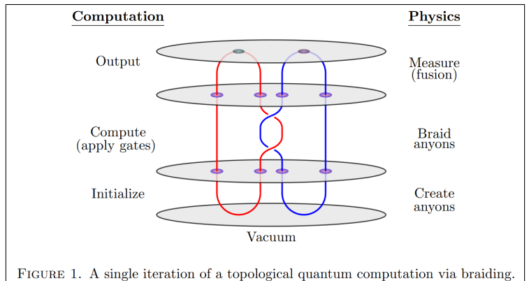
FIGURE 1. A single iteration of a topological quantum computation via braiding. Figure from Rowell ([109], following [108, Fig. 2]).
