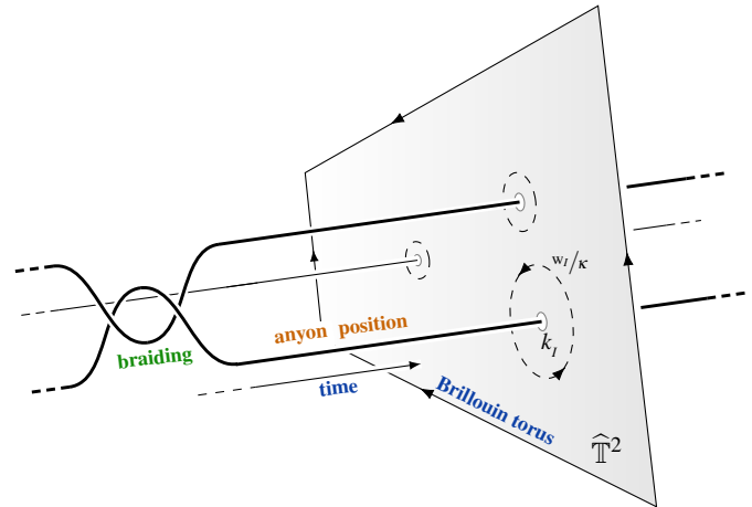
Figure 12 – Anyon braiding. Shown is a configuration of three points on a surface, evolving in time such that two of the points rotate around each other with their worldlines forming a braid.
