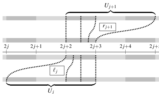
Figure 4.3: The situation in (4.324).
