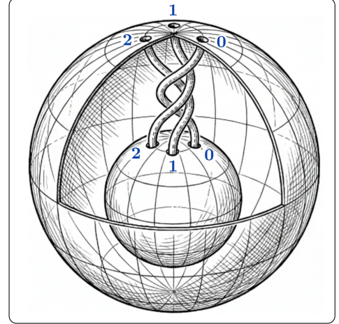
FIG. 2. Spherical braids (22) are braids of worldlines of punctures on the 2-sphere (cf. Fig. 1). These are almost the same as ordinary Artin braids of punctures in the plane. (Shown is the element b_1 b_2 b_1 b_2 b_1 ). The only difference being that on the sphere, the Artin braid (b_1 \cdots b_n)(b_n \cdots b_1) (where all punctures are fixed except one, which is circling the others) is topologically trivial.
