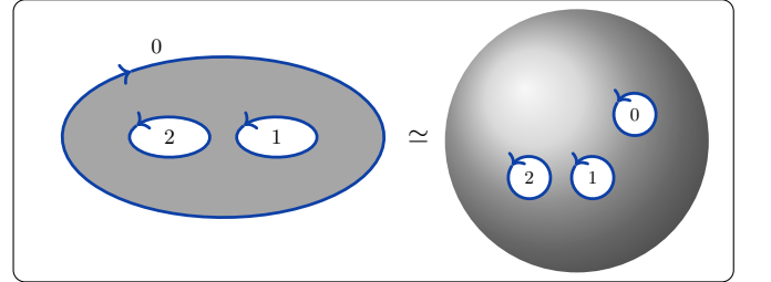
FIG. 1. A disk (hosting an FQH fluid) with n islands (punctures) is homeomorphic to a sphere with n+1 punctures. From the view of the complement bulk, all punctures are at infinity (19), which entails with (10) that magnetic flux does not enter here.
