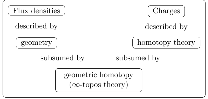
Figure 1: The geometric homotopy theory of \infty -topoi is the conceptual unification of geometry with homotopy theory, hence the theory of higher geometry . In our context, fluxes are (differential) geometric, charges are homotopical, and their unification happens through the construction of the phase space (§ 4.2.1) in the ambient cohesive \infty -topos (§ 2.3).
