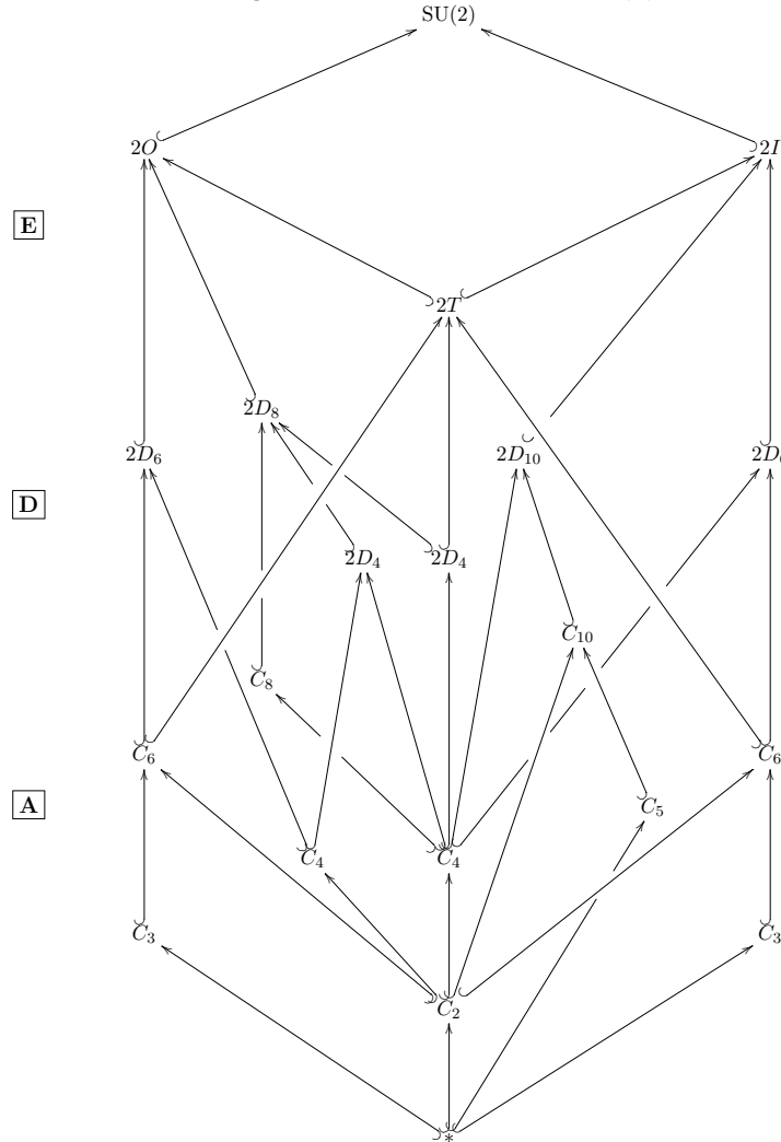
The full subgroup lattice of SU(2) under the three exceptional finite subgroups from Prop. A.1 (using the subgroup lattices from [Dok-2T, Dok-2O, Dok-2I]).
