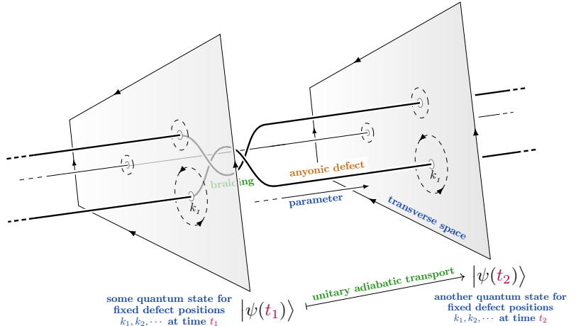
Figure A – Topological braid gates. Covariant flux quantum states on a sufficiently punctured surface, by their diffeomorphism equivariance (22), carry unitary representations of the braid group (24) of joint motions of the defects around each other, exhibiting the punctures as defect anyons .
