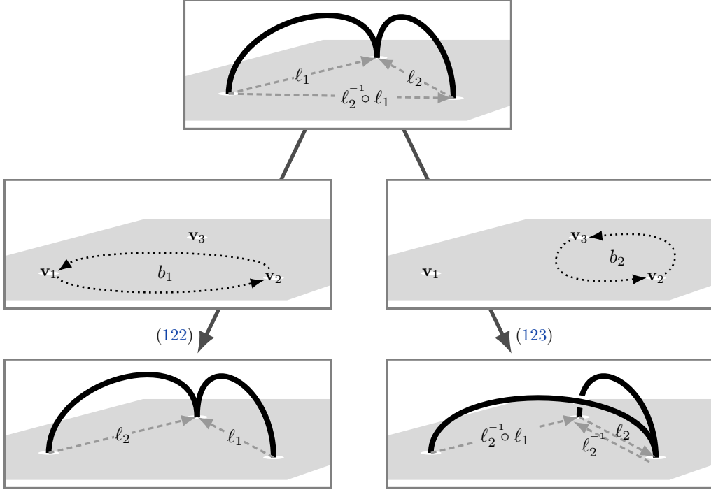
Figure S – Effect of braiding on compactification of punctured surface – proof of Prop. 3.45. Using that the homotopy type of the 1-point compactification (\Sigma_{g,b,n}^2)_{\cup\{\infty\}} of a punctured surface is obtained by attaching, for all j < n , an arc from the j th to the n th puncture (cf. the proof of Lem. 3.41), the above graphics shows the effect of the Artin generator (26) mapping classes b_i \in \text{Br}_n(\Sigma_{g,b}^2) \rightarrow \text{MCG}(\Sigma_{g,b,n}^2) on these arcs — and on the indicated generators \ell_j \in \pi_1((\Sigma_{g,b,n}^2)_{\cup\{\infty\}}, \infty) obtained after contracting the arcs to \{\infty\} — making manifest that after pushing each loop forward to \Omega S^2 this gives the “standard” representation (Def. 3.44) of the symmetric group \text{Sym}_n .
