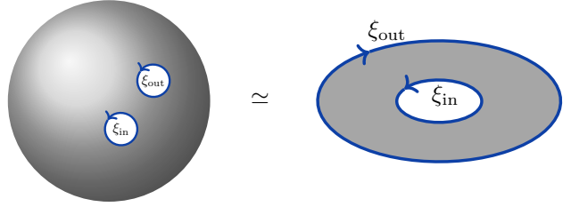
Figure OA. 2-Cohomotopical flux quanta on the open annulus (the 2-punctured sphere, cf. Fi. 1) have an observable \xi_{\text{in}}/\xi_{\text{out}} (142) to be interpreted as the (multiplicative) difference of phases associated with the two edges. Moreover, when this phase difference is not equal to \pm 1 then the (ground) state is 2-fold degenerate, with one basis state associated to each edge (141).
