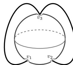
Figure A. There are several ways to attach arcs for n > 2 punctures in the above proof of Lem. 3.46, all equivalent in the resulting homotopy type. But for the analysis of braiding that follows in Thm. 3.50 it is useful (cf. Fig. S) to single out one puncture v_n and take the n - 1 arcs to connect this one puncture to each of the n - 1 remaining ones. The case g, b = 0 and n = 3 is illustrated on the right.
