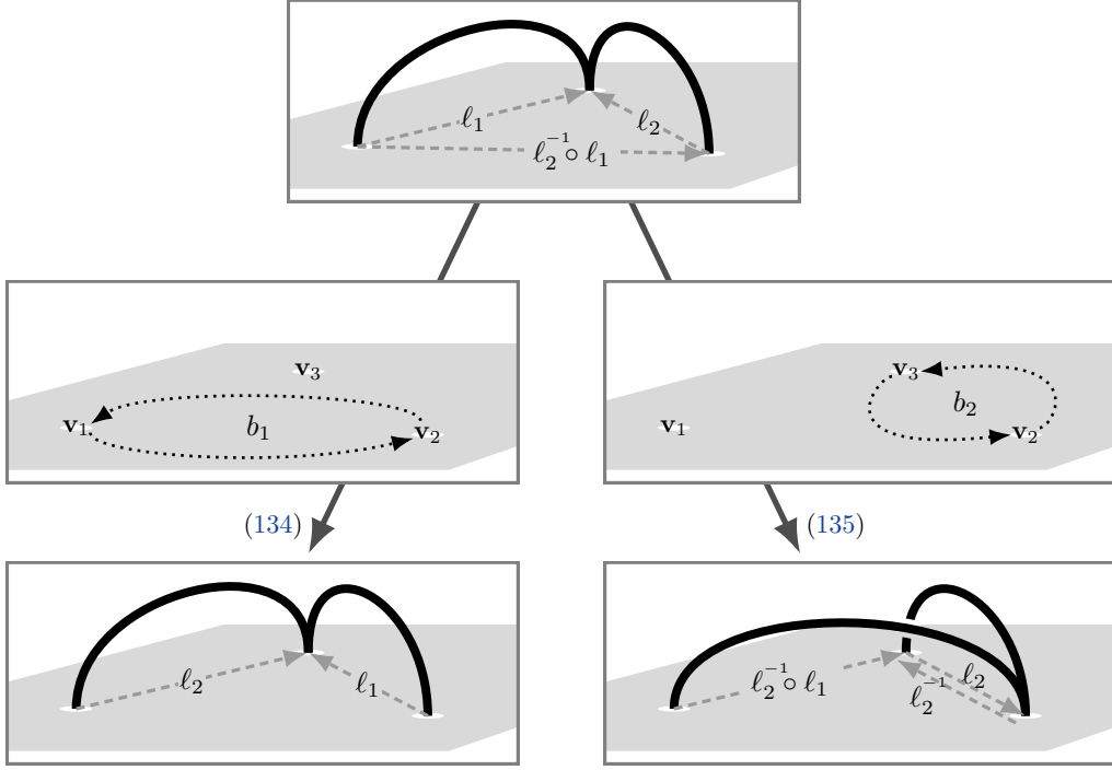
Figure S – Effect of braiding on compactification of punctured surface – proof of Thm. 3.52. Using that the homotopy type of the 1-point compactification (\Sigma_{g,b,n}^2)_{\cup\{\infty\}} of a punctured surface is obtained by attaching, for all j < n , an arc from the j th to the n th puncture (cf. the proof of Lem. 3.48), the above graphics shows the effect of the Artin generator (26) mapping classes b_i \in \text{Br}_n(\Sigma_{g,b}^2) \rightarrow \text{MCG}(\Sigma_{g,b,n}^2) on these arcs — and on the indicated generators \ell_j \in \pi_1((\Sigma_{g,b,n}^2)_{\cup\{\infty\}}, \infty) obtained after contracting the arcs to \{\infty\} — making manifest that after pushing each loop forward to \Omega S^2 this gives the “standard” representation (Def. 3.51) of the symmetric group \text{Sym}_n .
